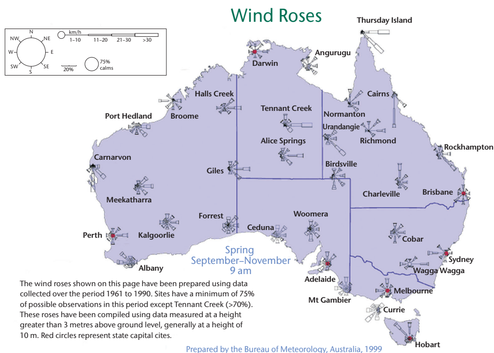
Figure 6.12. Example of a symbolic map display of wind
