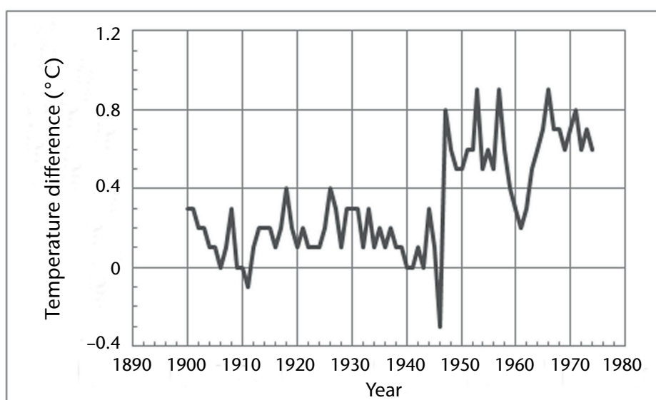
Figure 5.2. Example of a difference time series
