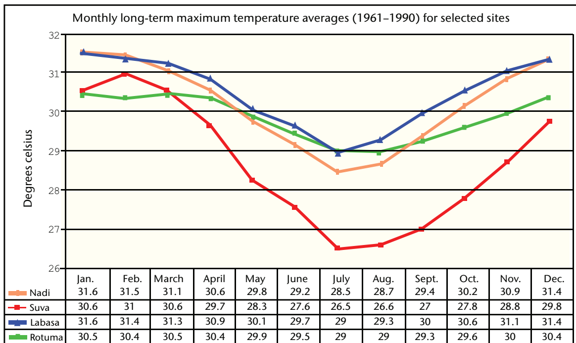
Figure 6.7. Example of a line graph and table of temperature values for multiple stations
