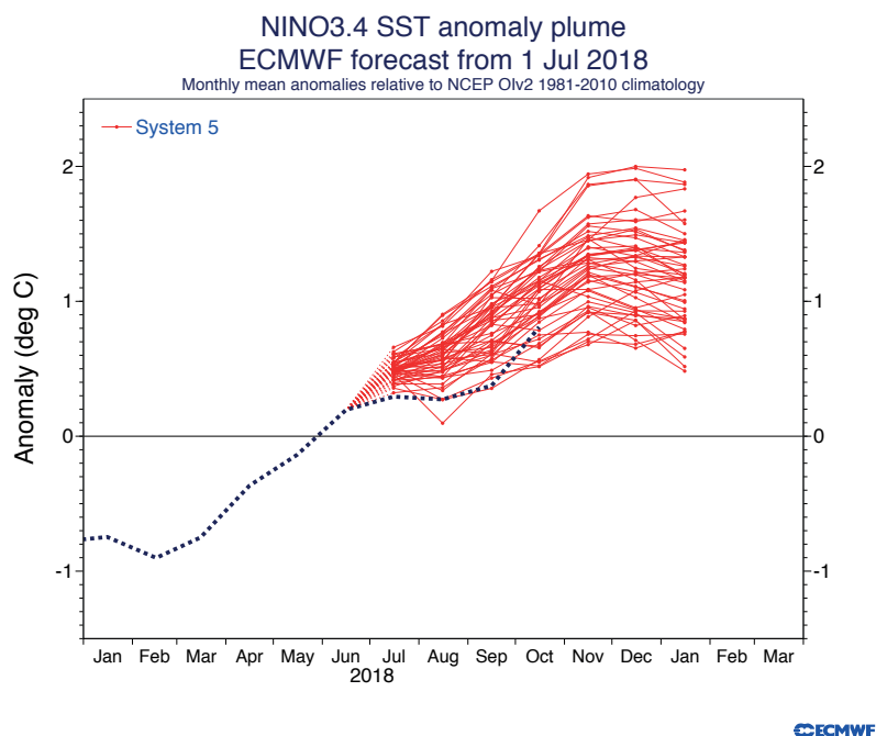
Figure 6.3. Example of plumes representing the spread of a seasonal forecast (e.g. El Niño plumes)
