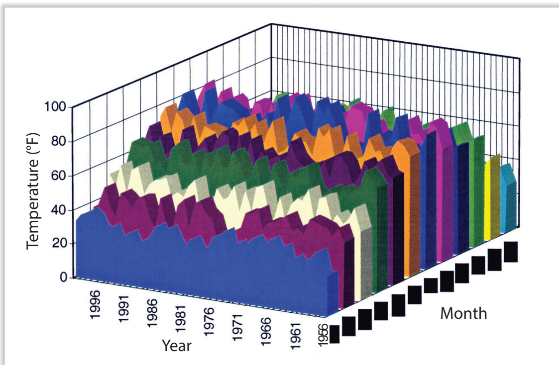
Figure 6.11. Example of a three-dimensional display emphasizing time series of monthly values for a given year
