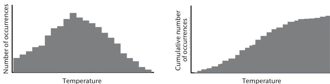
Figure 4.1. Frequency distribution (histogram) Figure 4.2. Cumulative frequency distribution
