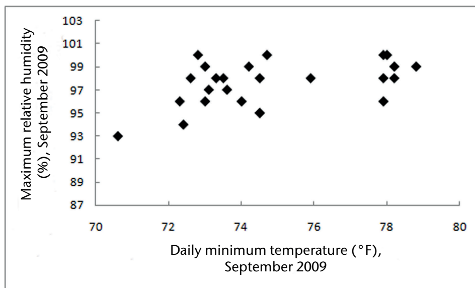
Figure 4.17. Scatter diagram with strong positive correlation
