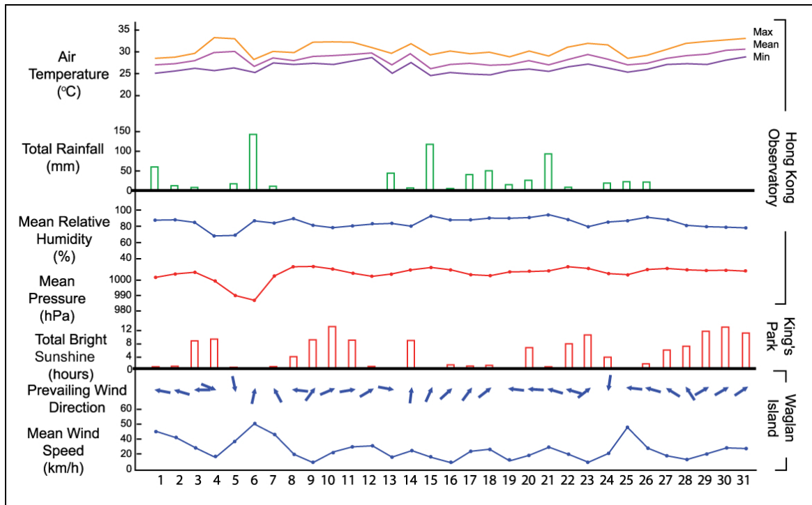
Figure 6.6. Example of a graphical display of daily values of several elements
